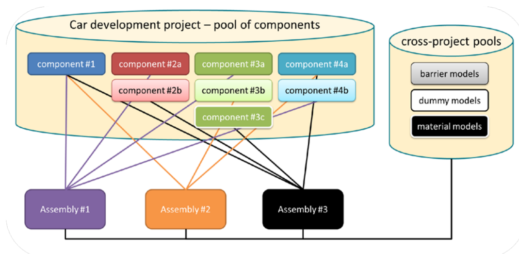
Figure 3: Assembling different crash simulation models
