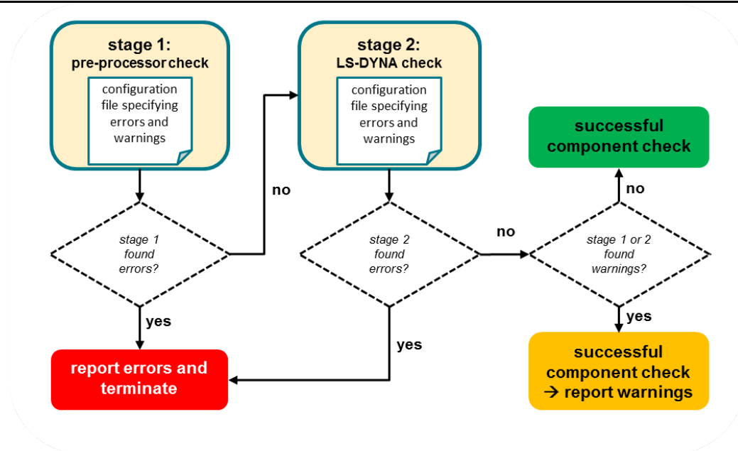
Figure 2: Program flow of check environment DynaCheck
